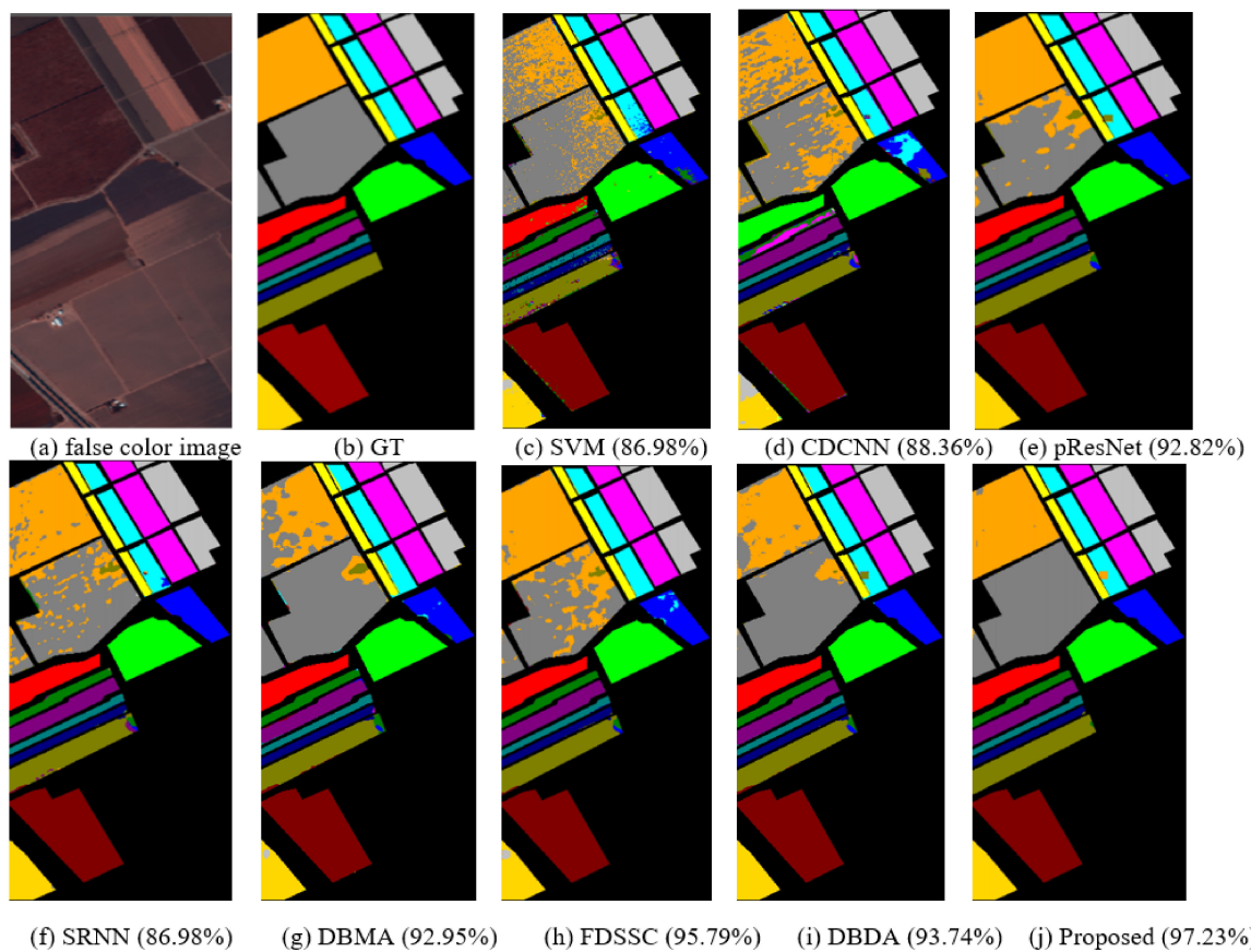
Figure 9. Classification maps of SV data set using 0.5% training samples: (a) false color image, (b) ground truth map (GT) and (c–j) the classification map and overall accuracy of different algorithms.
